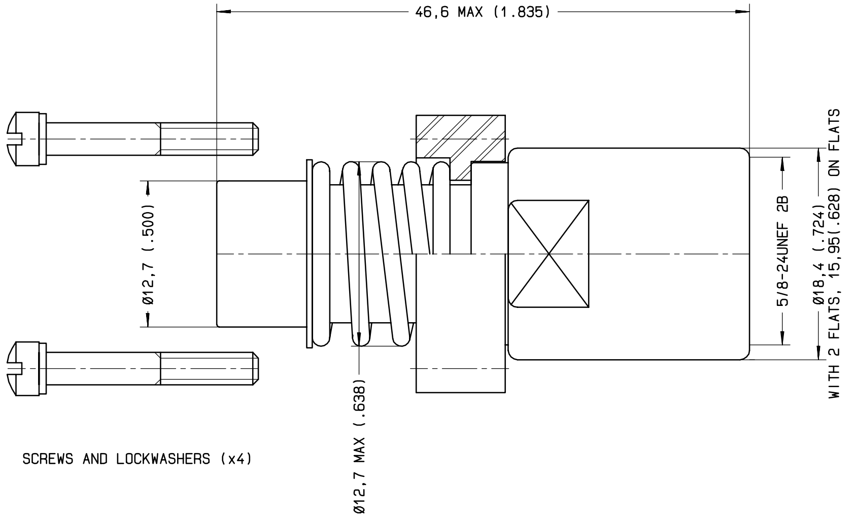
OUTER CONTACT SUB ASSY. AND RETAINING BLOCK
